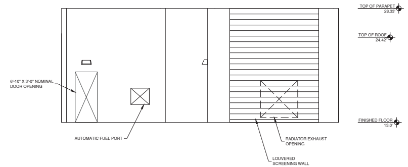
SOUTH ELEVATION 1/4" = 1'-0"
