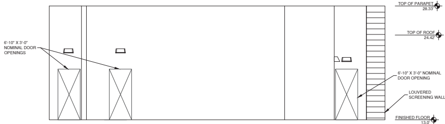
WEST ELEVATION 1/4" = 1'-0"
