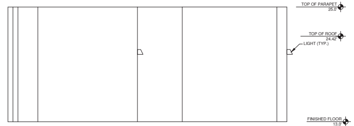
NORTH ELEVATION 1/4" = 1'-0"
