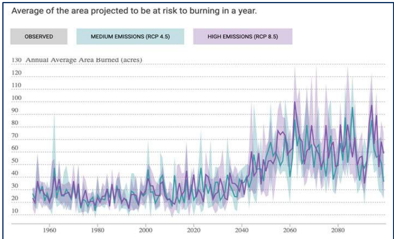
Figure 17-6. Annual Average Area Burned, Model Simulation
